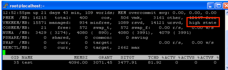
Figure 7: Host free memory state in esxtop
