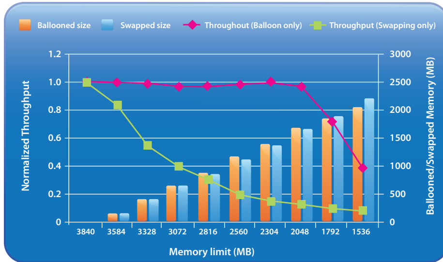
Figure 11: Performance of Swingbench when using ballooning vs. swapping
