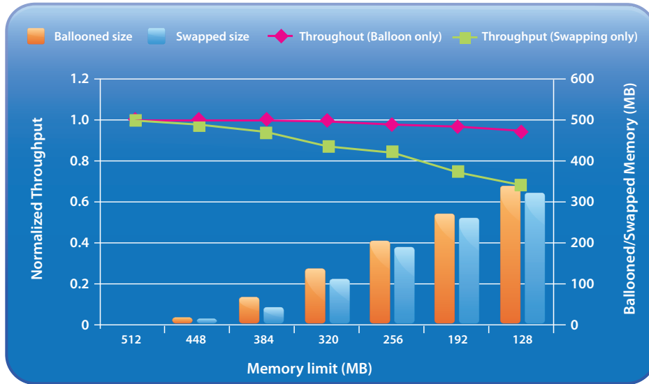
Figure 10: Performance of kernel compile when using the ballooning vs. the swapping
